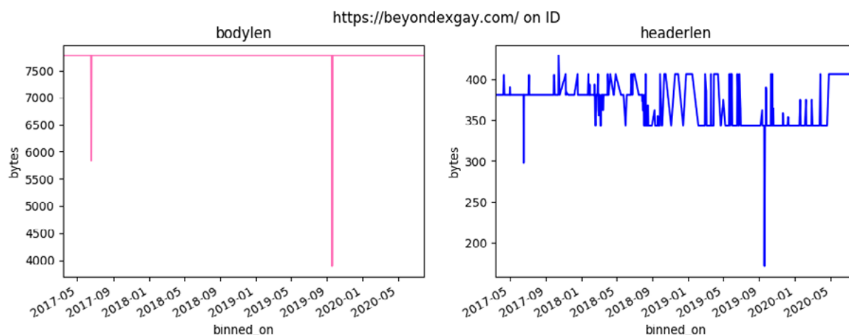
Figure 5: A graph of body and header length over time for the beyondexgay.com site in Indonesia. The two spikes here are outliers that would have been investigated further.
